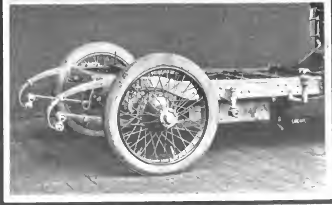
Rear axle of the Lanchester showing the differential cover removed Rear axle of the Panhard—D, differential housing; T, axle casing Showing general design of Crossley double-drive rear axle Rear portion of Wolseley 16-20 chassis, showing spring arrangement
